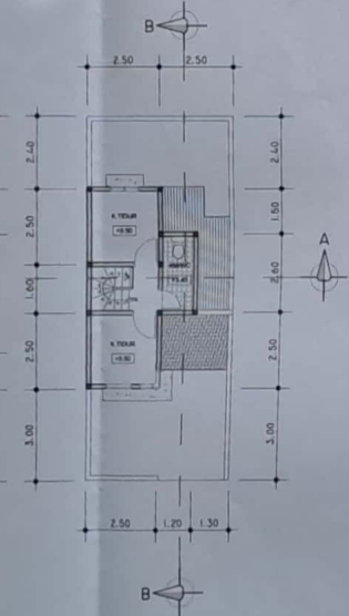
DENAH LT.2 Skala 1:100
